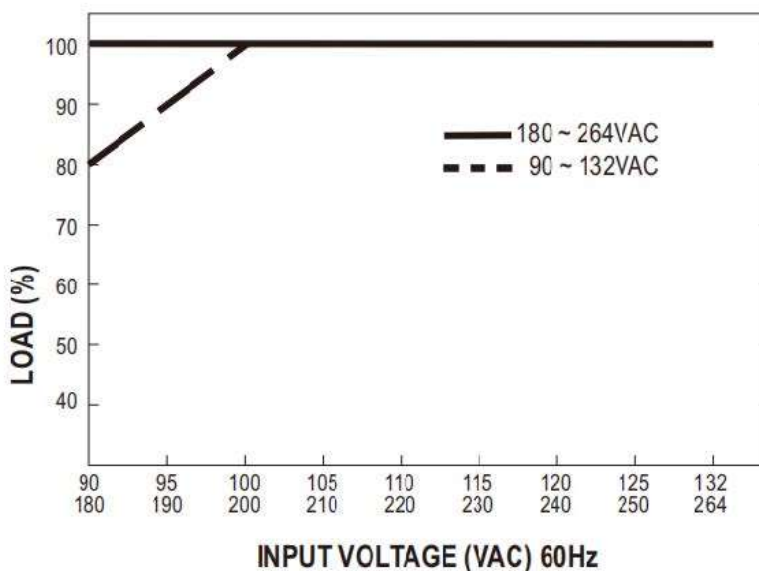
Figure 2) AC Input Voltage Derating / Output Load Derating Versus Input Voltage
